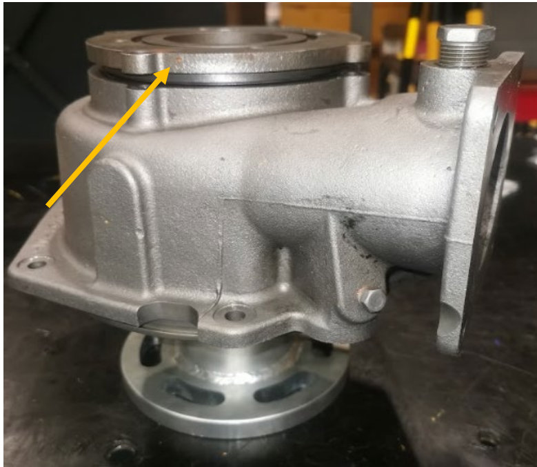
Figure 6: Impeller cover with the multi-purpose tool.
